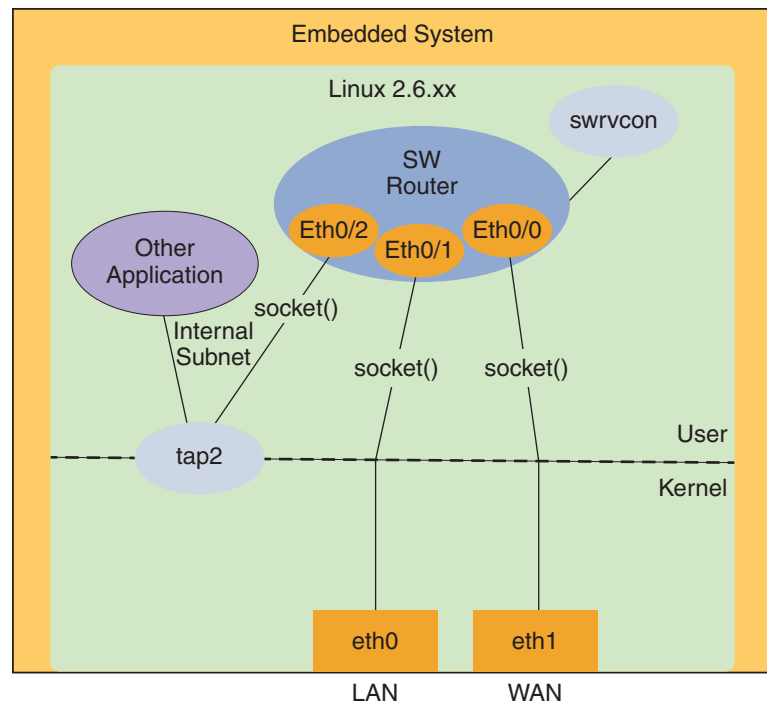
Figure 1-1 Interactions between Cisco 5921 ESR Components
